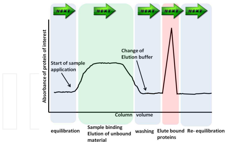
Fig. 1. Typical affinity chromatography purification
