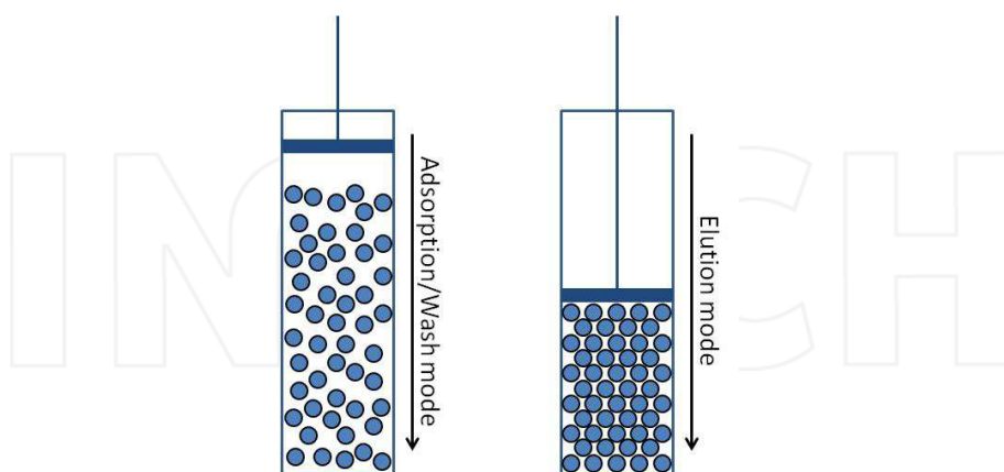
Fig. 3. Expanded-bed chromatography. In this type of chromatography, elution is performed in a normal packed-bed, but during the adsorption-wash step, the flow is reversed and the column bed expanded. This allows for particulate contaminants to pass freely through the column and prevent column clogging.
