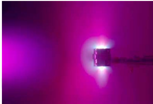
Fig. 22. Typical flow around miniature MPS during quasi-steady operation (discharge current of SWS is 8 kA ( H_2 :0.4 g/s), and discharge current of MPD_Inf is 4.2 kA ( H_2 :0.05 g/s)).
