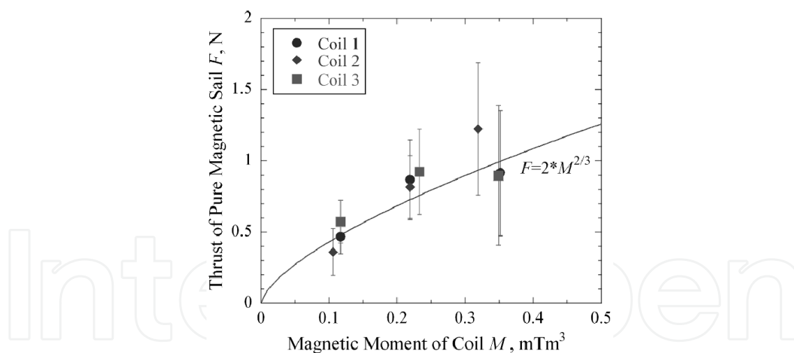
Fig. 16. Thrust vs. magnetic moment in the case of MagSail; SWS was operated for hydrogen plasma flow ( u_{sw}=47 km/s, n=1.8 \times 10^{19} m ^{-3} ), and three types of coils (radius=25 mm (coil 1,2) or 35 mm (coil 3)) are positioned at X=0.6 m.
