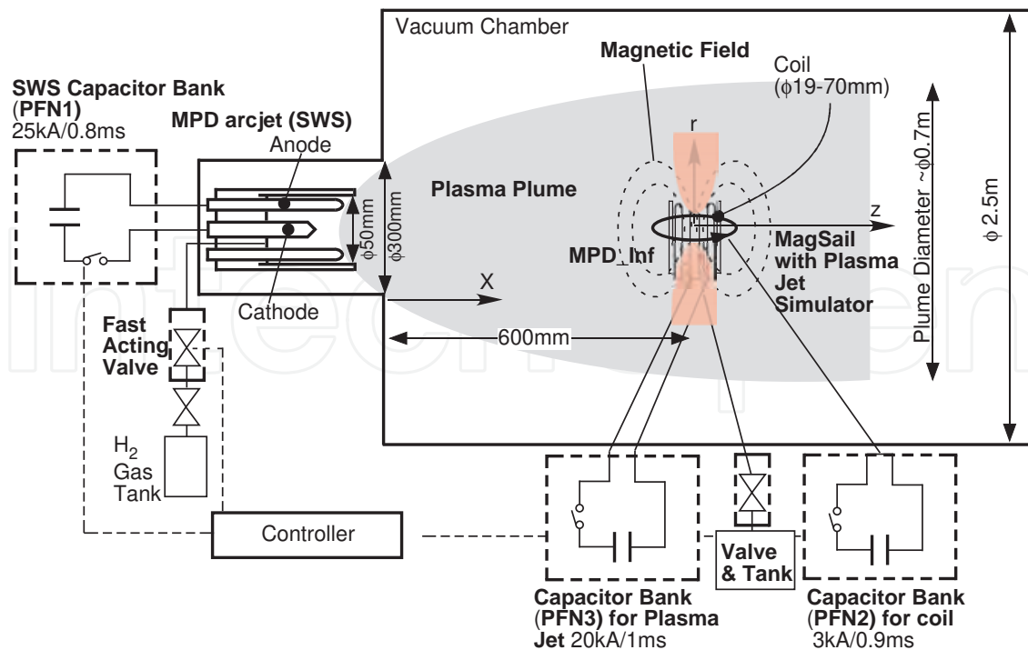
Fig. 20. Experimental setup for magnetoplasma sail (MPS).
