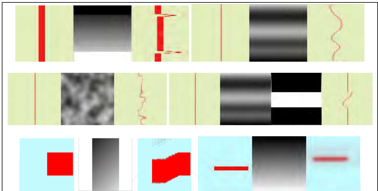
Fig. 33. Convolution filters
