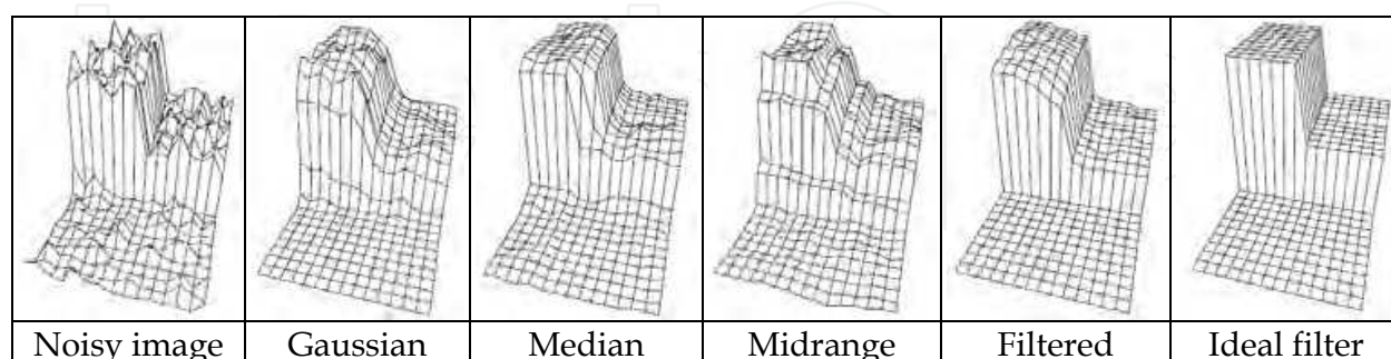
Fig. 30. Filters responses
