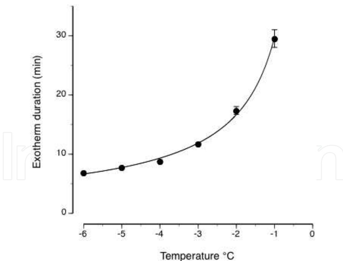
Fig. 1. The effect of temperature on the exotherm duration of 10\mu\text{l} suspensions of the Antarctic nematode Panagrolaimus davidi . N = 4 , bars are standard errors. The line is the fit to the equation f(x) = \exp(3.39) * (x^{-0.83}) , R^2 = 0.996 . Redrawn from (Wharton et al., 2002).
