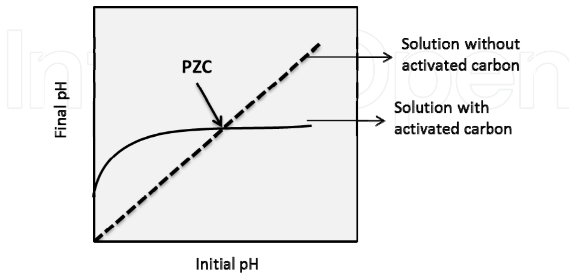
Figure 2. PZC measurement determined in several solutions at different initial pHs.
