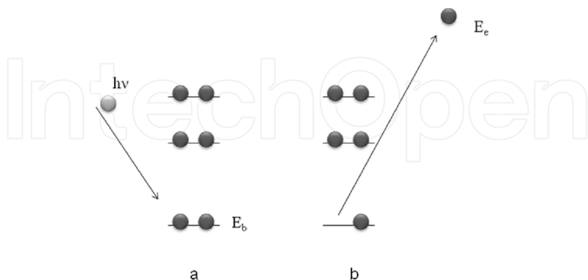
Figure 4. Mechanism of X-Ray Photoelectron Spectroscopy.
