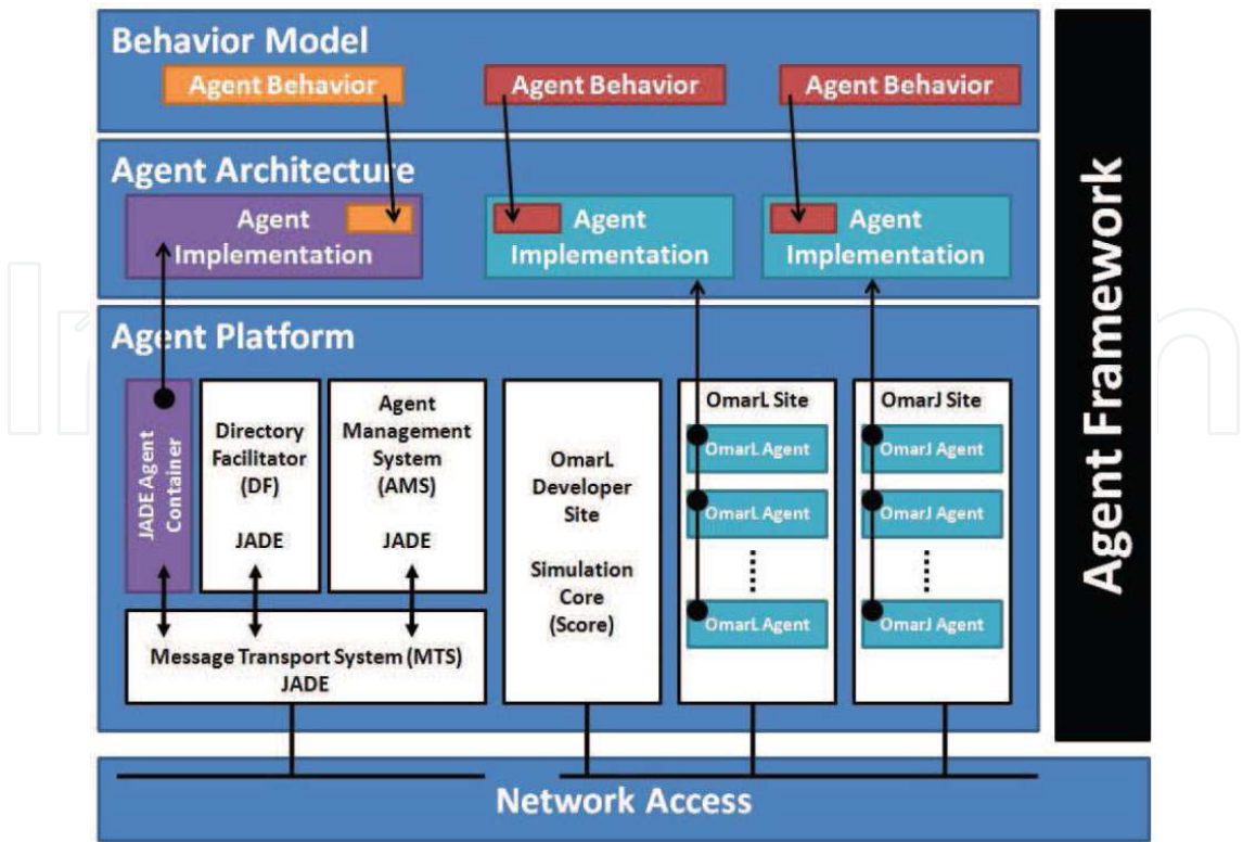
Fig. 2. Description of Agent Framework.
