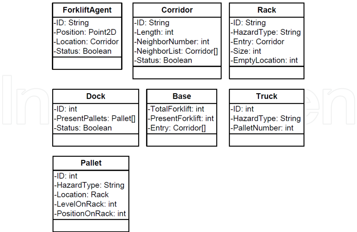
Fig. 7. Classes used to reproduce the activities of storage in a warehouse of chemical substances.
