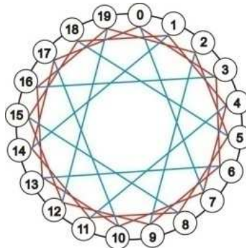
Fig. 6. Modified chordal ring CHR5\_a(20; 3,7)
