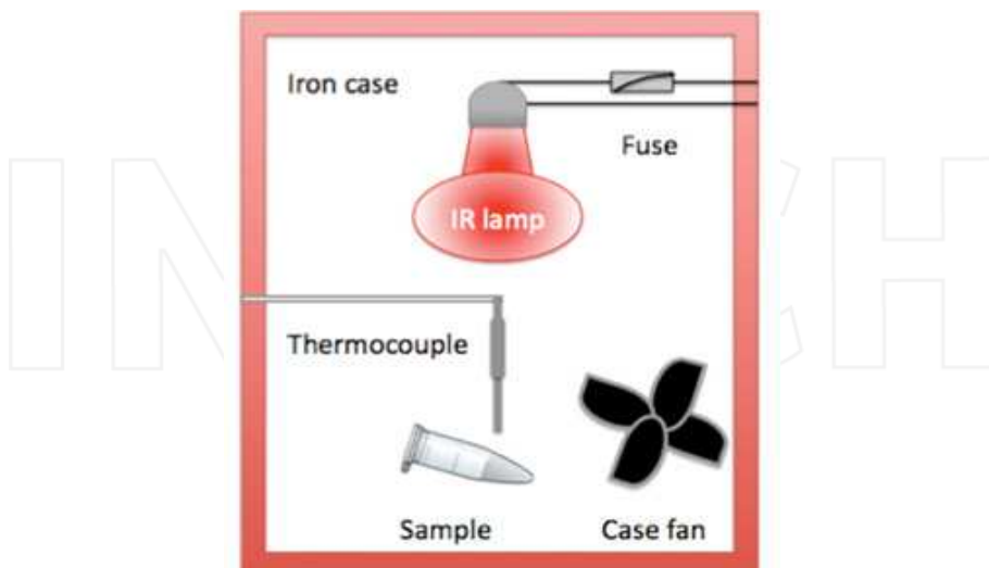
Fig. 4. Schematic diagram of the IR-assisted proteolysis system, adapted from (Wang et al. 2008).
