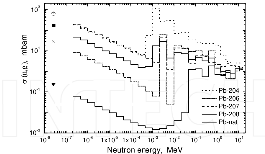
Fig. 1. Microscopic cross sections of radiation neutron capture \sigma(n, g) by stable lead isotopes and by natural mix of lead isotopes taken from the ENDF/B-VII.0 library. Cross sections are represented in the ABBN-93 system of 28 neutron energy groups.
