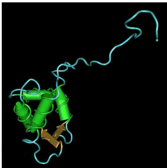
Fig. 4. Structure of the C-terminal Ef-hand domain of human cardiac sodium channel.
