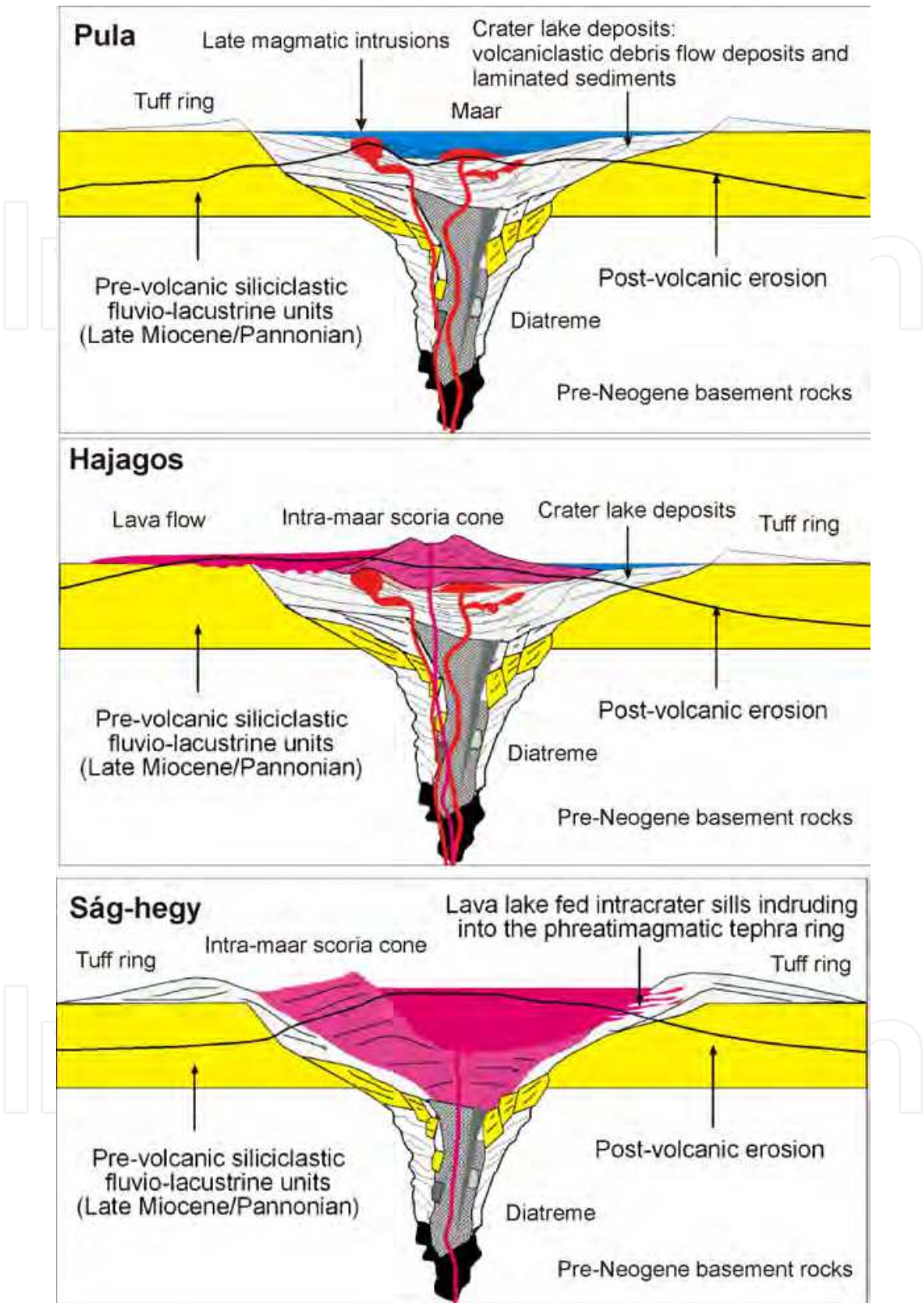
Fig. 10. Theoretical cross-sections of complex maar volcanoes reconstructed on the basis of preserved pyroclastic rocks, their texture and distribution patterns. A combination of crater lake sedimentation and/or magmatic crater filling successions are reconstructed on the basis of preserved 3D facies architecture of volcanic rocks and their textural characteristics.
