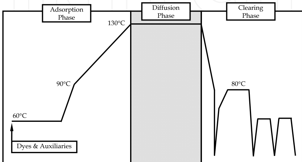
Fig. 16. Phases of exhaust dyeing of polyester.
