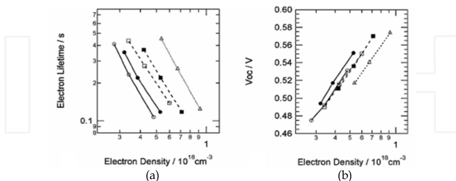
Fig. 15. (a) Electron lifetime, and (b) V_{oc} , as a function of electron density in the TiO 2 film for porphyrin DSSCs after 0 mins (circles), 5 mins (squares) and 30 mins (triangles) of a phosphonic acid surface treatment. Figure taken from (Allegrucci, Lewcenko et al., 2009) and reproduced by permission of The Royal Society of Chemistry.
