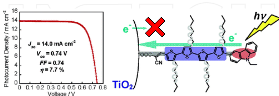
Fig. 14. PV parameters and an illustration of a carbazole dye with long alkyl chains to stop the redox mediator reaching the semiconductor surface. Figure taken from (Koumura, Wang et al., 2006) and reproduced by permission of The American Chemical Society.
