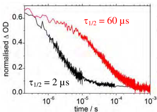
Fig. 13. Transient absorption kinetic traces recorded at 700 nm for porphyrin-sensitized TiO_2 films covered with acetonitrile electrolyte in the absence (red) and presence (black) of an I^-/I_3^- redox mediator. The films were photoexcited by nanosecond pulses at 532 nm.
