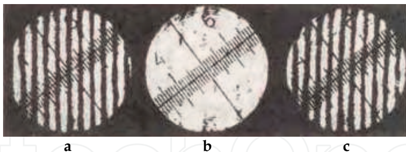
Fig. 27. The interference pattern with \lambda/2 anisotropic phase plate after polarizer
