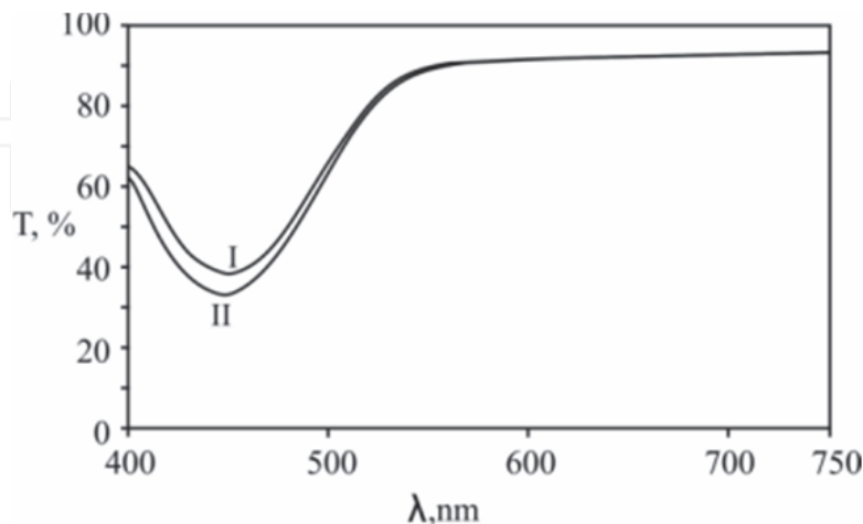
Fig. 1. Spectral transmittance characteristics of azobenzene
