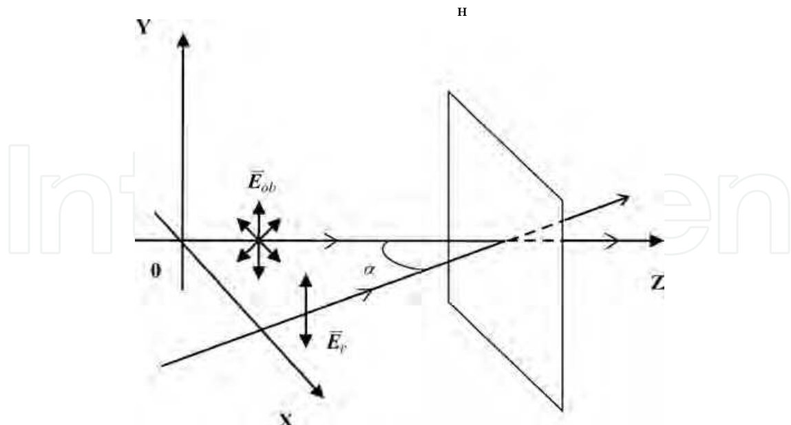
Fig. 7. The scheme of holographic recording
