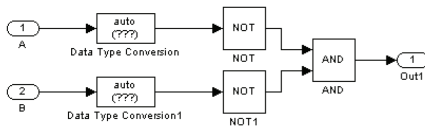
Fig. 12. Block for control of writing
