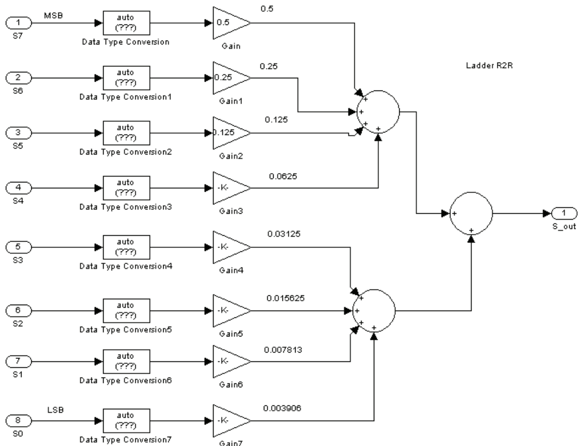
Fig. 7. R-2R ladder network implemented as subsystem
