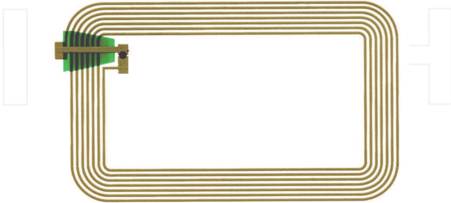
Fig. 2. Antenna design (13.56MHz, 45mm x 76mm) for the study
