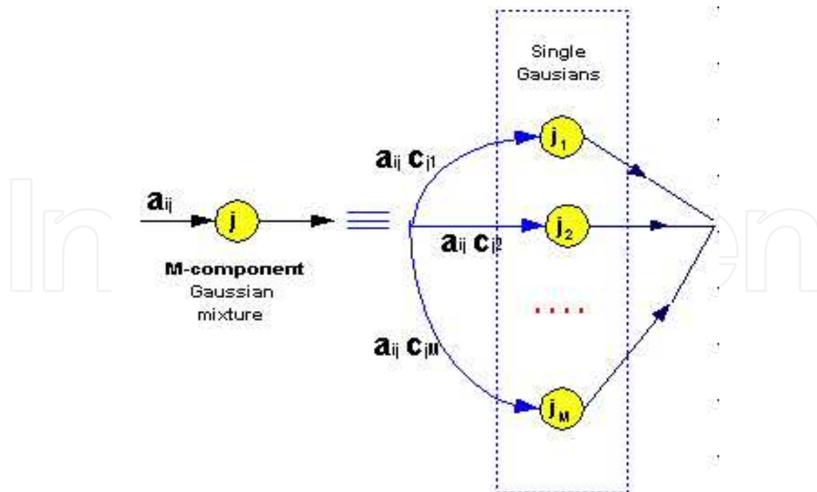
Fig. 4.4 Baum-Welch algorithm
