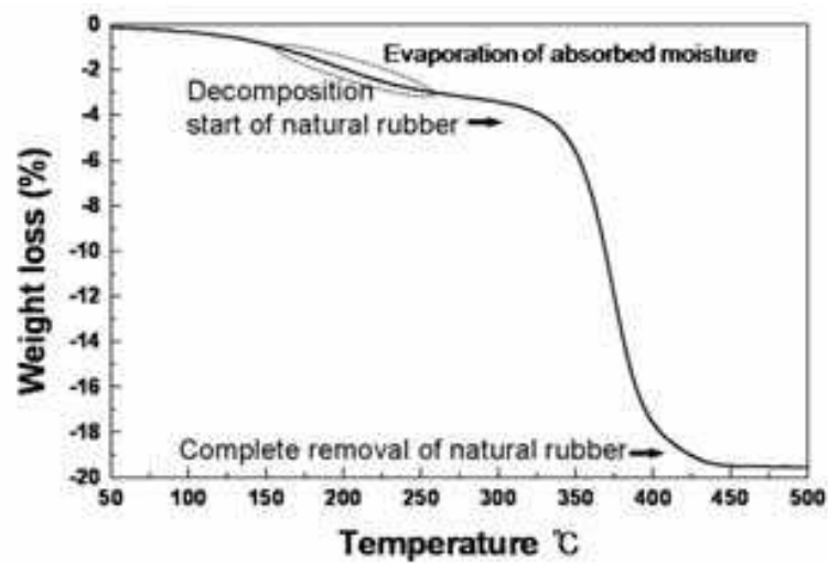
Fig. 2. TGA curve of Al-NR-CNT precursor.
