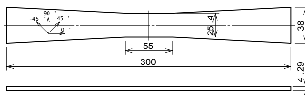
(a) NHT specimen for static tests
