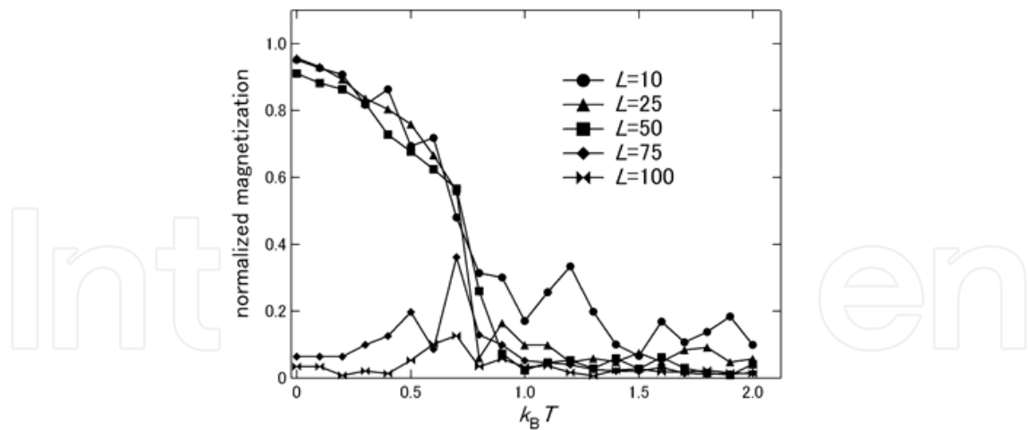
Fig. 5. Temperature dependence of normalized magnetization M for different size square clusters.
