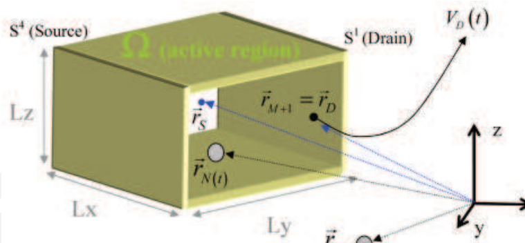
Fig. 8. The electrostatic potential V_D(t) (due to internal and external electrons) measured on the surface S^1 at position \vec{r}_D and time t by an additional probe charge q_{M+1} situated on the boundary \vec{r}_D \equiv \vec{r}_{M+1} \in S^1 .
