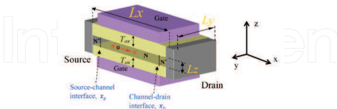
Fig. 9. Schematic representation of the quantum wire double gate FET.
