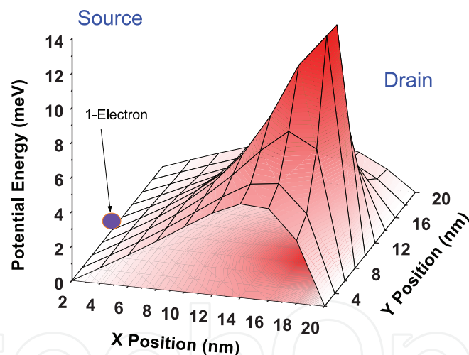
Fig. 4. Potential energy profile of the 1-electron, \bar{W}_1(\vec{r}_1, t) , with the “many-electron” algorithm in the plane X-Y of the active region \Omega = (20 \text{ nm})^3 at z=6\text{nm} at 0.4 fs. The solid point is the 1-electron position. Reprinted with permission from G. Albareda et al., Phys. Rev. B. 79, 075315 (2009). ©Copyright 2009, American Physical Society.
