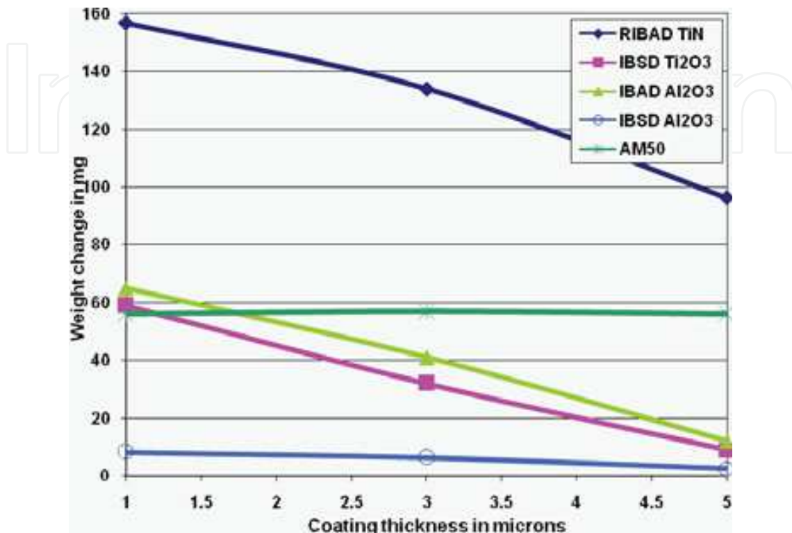
Fig. n.3.12. Weight change of AM50 substrates coated with various thickness and subjected to 48 hours immersion in acidified 5% NaCl solution, following the procedure described in section 3.2.2.4
