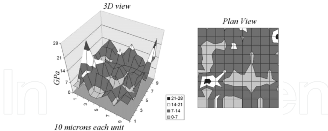
Fig. n.2. Nano hardness measurements on IBAD \text{Al}_2\text{O}_3 coating with I/C ratio of 0.3 to determine the hardness of the phases present.
