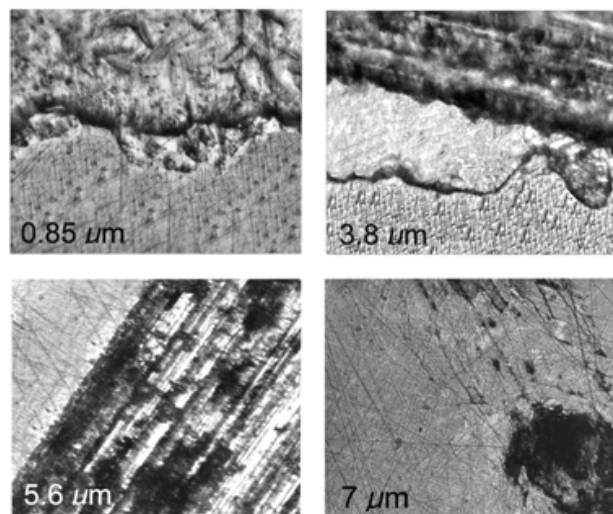
Fig. n.3.9. Optical micrographs of \text{Al}_2\text{O}_3 coatings deposited with an I/C of 0.3 and different coating thickness, showing wear tracks produced by running the pin-on-disc test until failure
